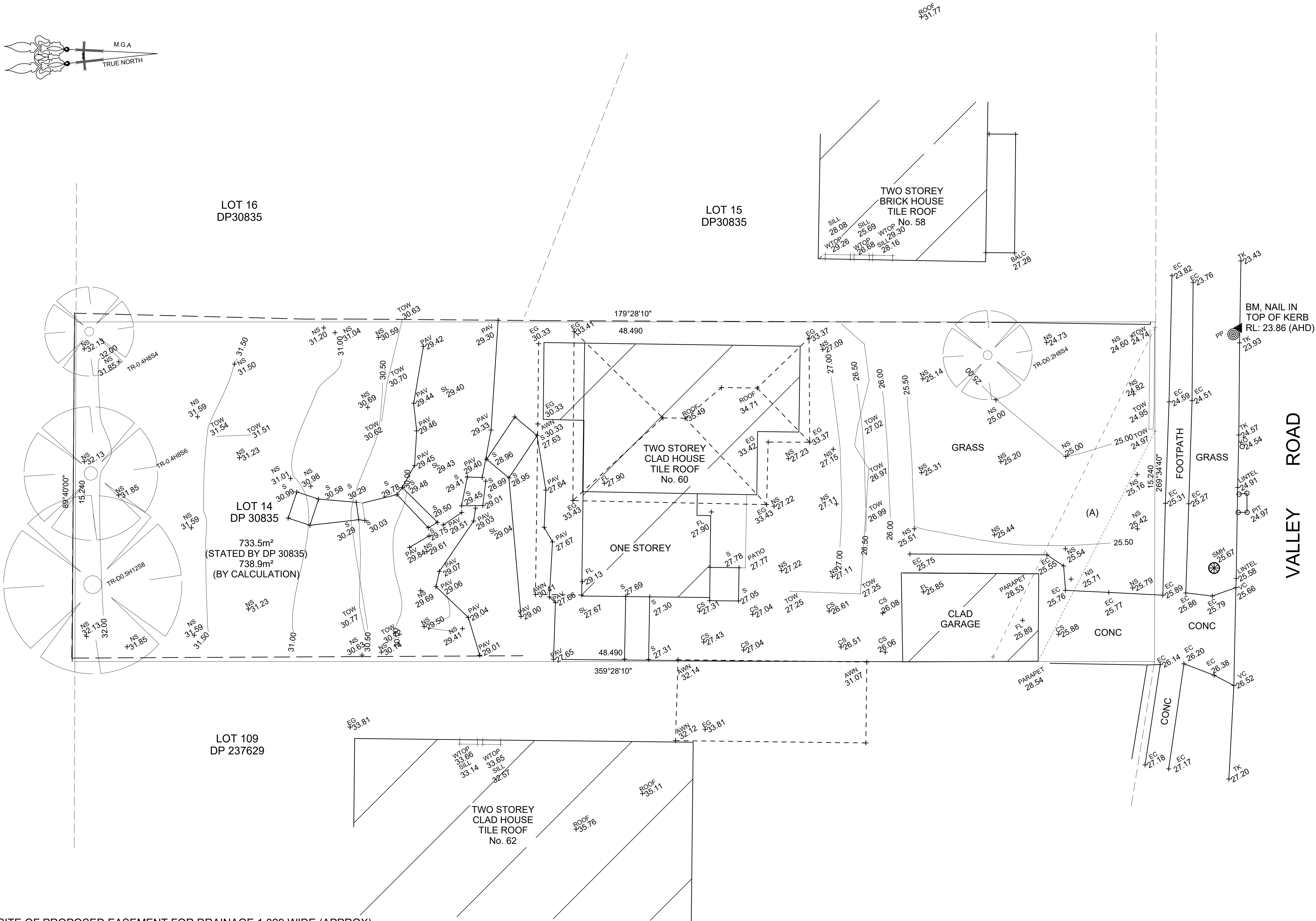
(A) - SITE OF PROPOSED EASEMENT FOR DRAINAGE 1.829 WIDE (APPROX)
